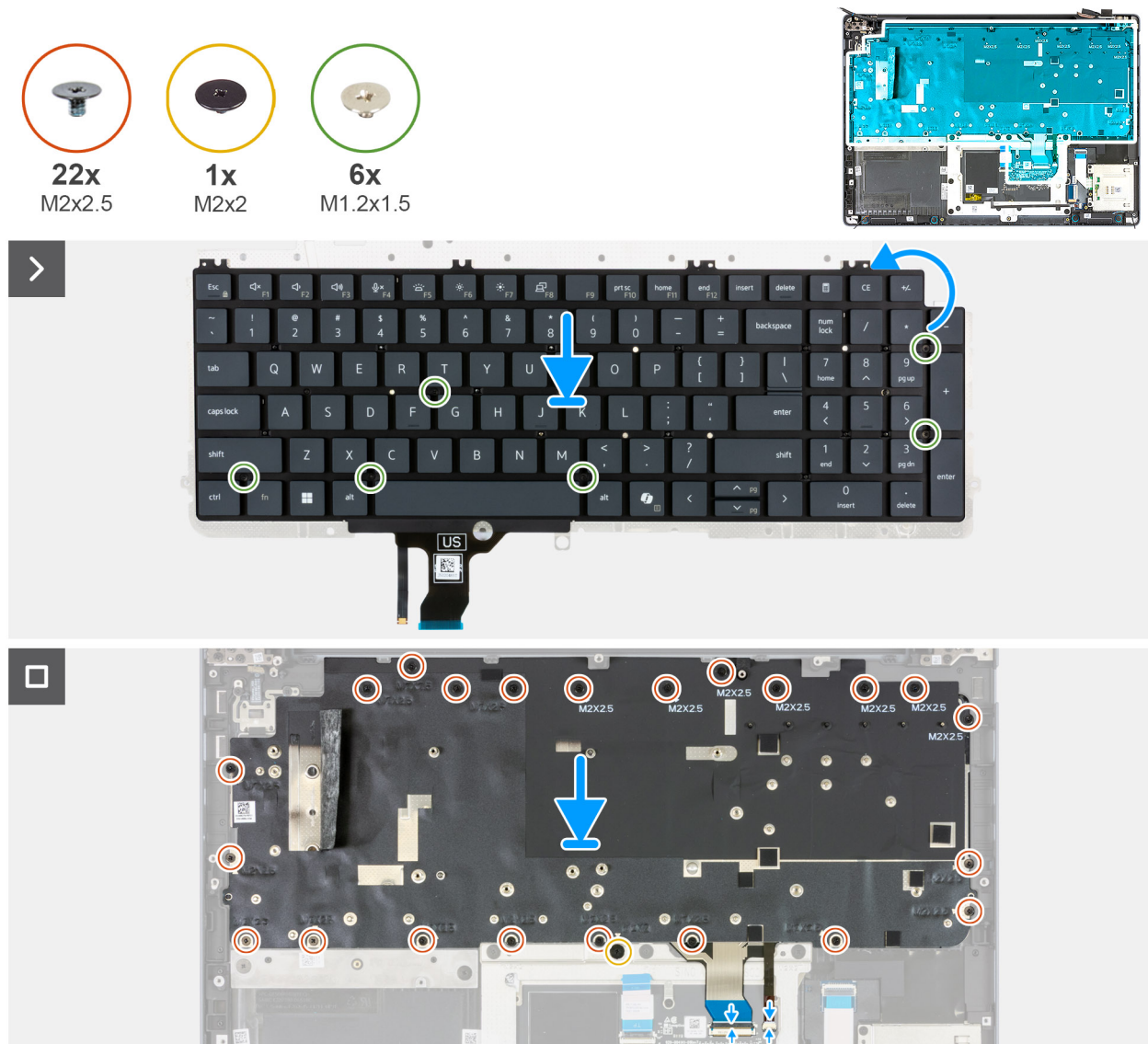
Figure 123. Installing the keyboard
