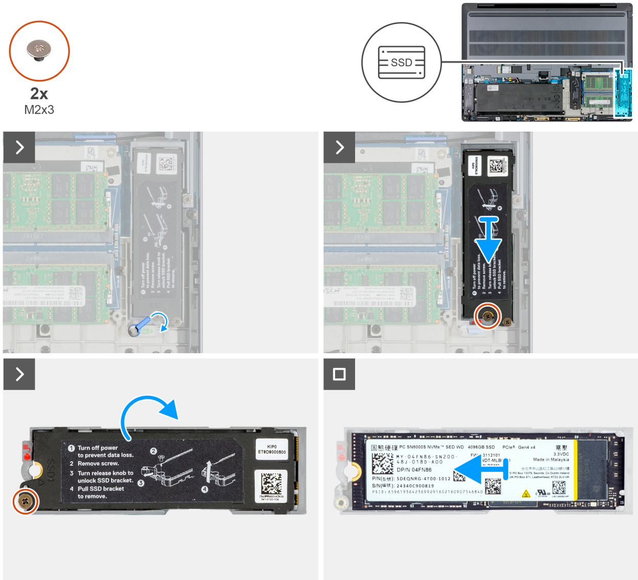
Figure 32. Removing the M.2 2280 SSD from slot 1 (SSD1)
