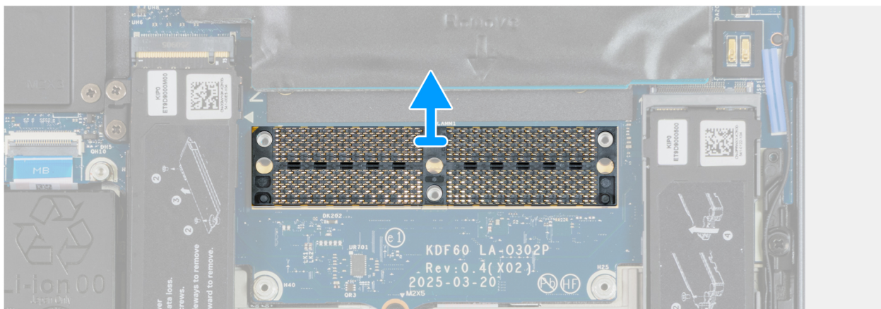
Figure 72. Removing the memory connector
