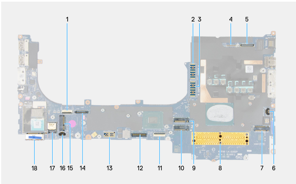
Figure 111. System-board connectors
