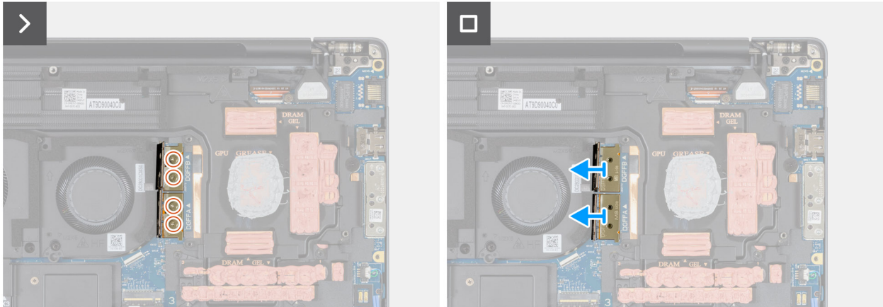
Figure 55. Removing the discrete FPC beam connector
