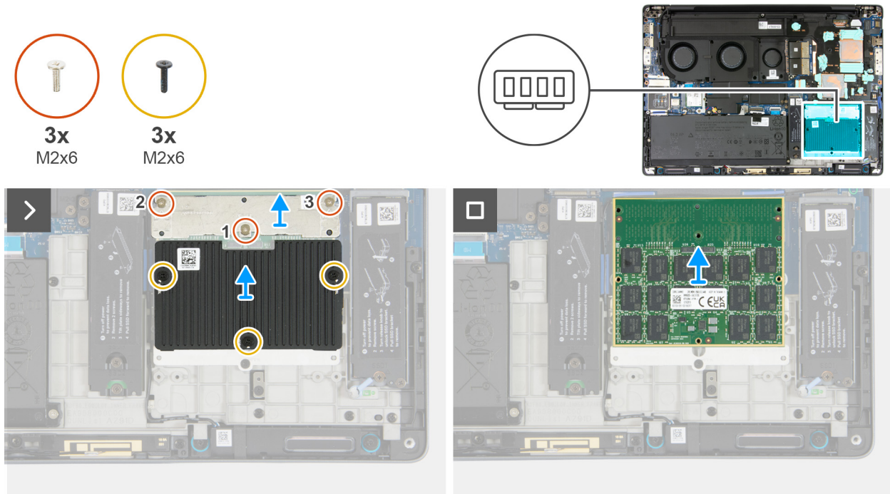
Figure 62. Removing the CAMM module (dual-channel)
