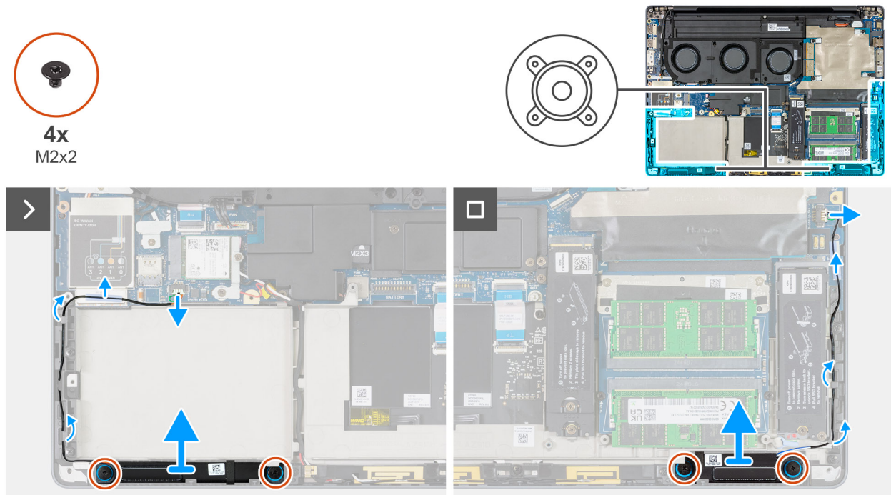
Figure 84. Removing the speakers
