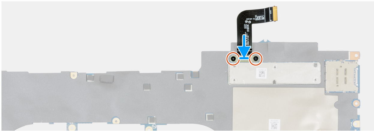
Figure 121. Installing the USH board cable
