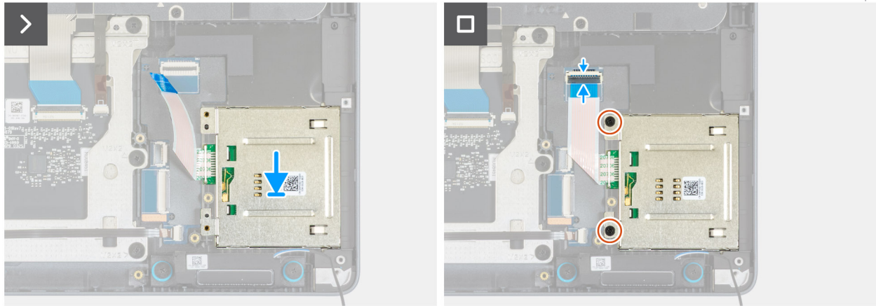
Figure 125. Installing the smart card reader
