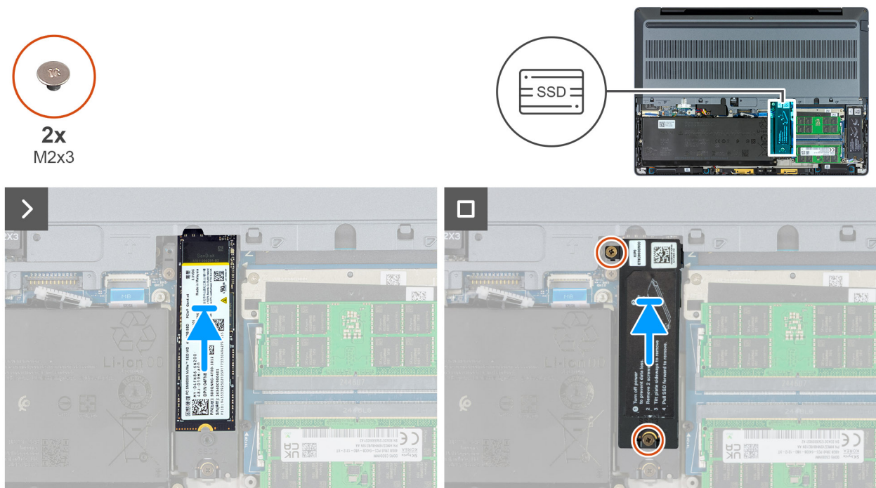
Figure 35. Installing the M.2 2280 SSD in slot 3 (SSD3)
