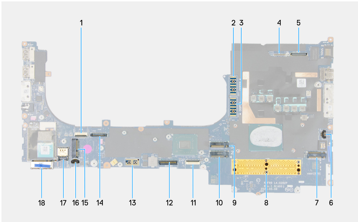
Figure 115. System-board connectors
